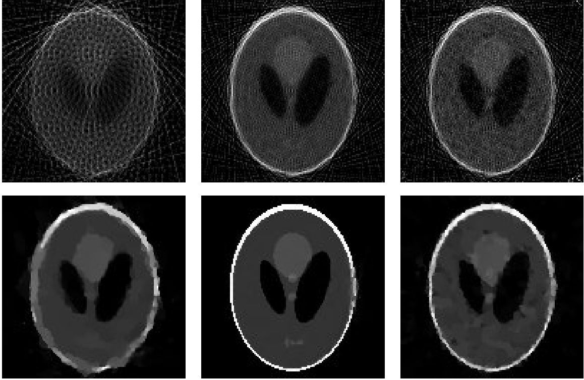
Figure 3.26: Reconstructions of the Logan-Shepp Phantom for a maximum tilt angle of \Theta_{max} = 85^\circ . First column: n_a = 20 , H = 1/32 , no noise added: Second and third column: n_a = 40 , H = 1/64 , without noise and with noise ( \sigma = 2 , e_{rel}(\mathbf{d}) = 0.053 ), respectively; First row: Kaczmarz reconstructions; Second row: TV-reconstructions (with \mu = 0.0001 , \mu = 0.001 , and \mu = 0.05 , from left to right).
