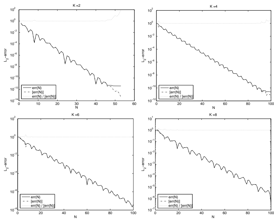
FIGURE 6.2. True error compared to error estimator for projection P_K u_0
