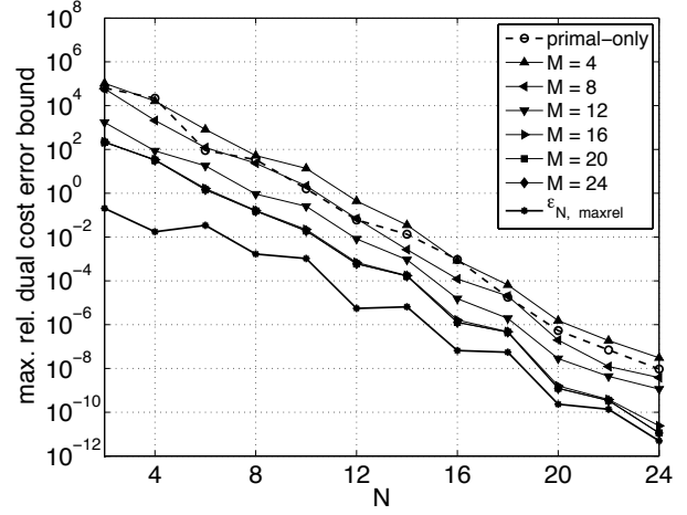
FIGURE 4. Maximum relative cost functional error, primal-only error bound \Delta_{N,\max,\text{rel}}^{J,*} , and primal-dual error bound \Delta_{N,M,\max,\text{rel}}^{J,*} as a function of N and M .
