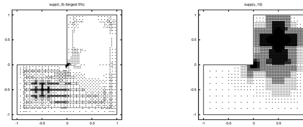
Fig. 5. Largest (in modulus) 5% of coefficients appearing in the primal residual vector and index set \mathcal{A}_{10} generated in Example 2.
