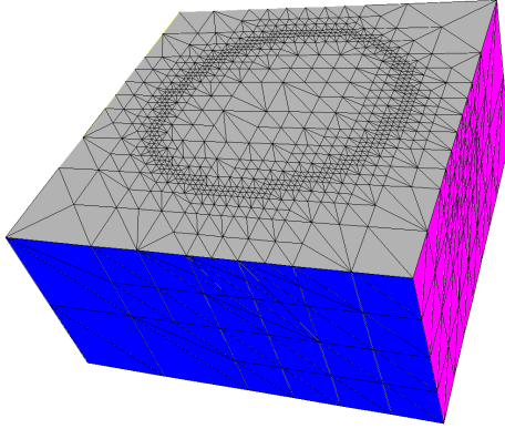
FIG. 6.1. Lower half part of the 4 times refined mesh \mathcal{T}_4 .
