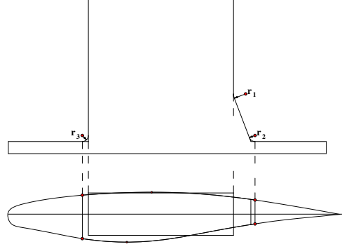
Fig. 6 Top and front view of mounting unit with continuation
