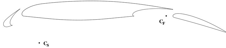
Fig. 17 Three element high lift configuration. The dots mark the rotation centers for the slat and flap riggings.
