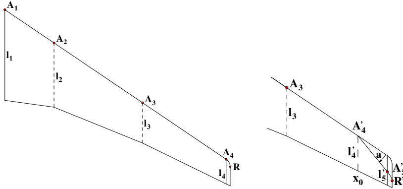
Fig. 5 Shear Plan of the multi-parted back-swept wing – winglet modifications on right hand side, see Section 2.4. For later reference: The coordinate in span direction (i.e. the horizontal direction in the sketch) is the x -coordinate, the vertical direction is described by the y -coordinate.
