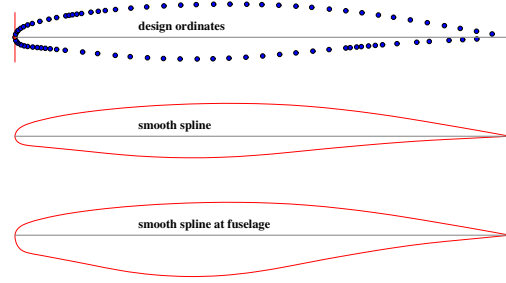
Fig. 4 Design ordinates, spline ( rt = 11\% ) and spline at fuselage ( rt = 15\% ). For later reference: the horizontal direction in this sketch corresponds to the y -coordinate of our 3D-coordinate system. The vertical direction corresponds to the z -coordinate.
