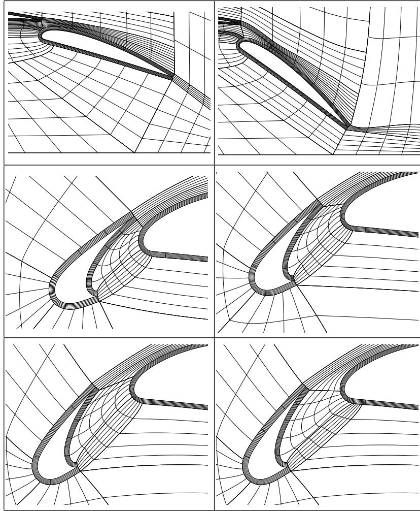
Fig. 19 Detailed viewed at the slat and flap. First row: grid around slat in initial configuration (left) and rotated 20^\circ clock-wise. Second row: grid around flap in starting configuration (left and rotated counter-clockwise by 6^\circ ). Third row: same grid rotated 12 degrees counter-clockwise with vertices rigidly fixed to the offset curves (left) and vertices allowed to move on the offset curve (right).
