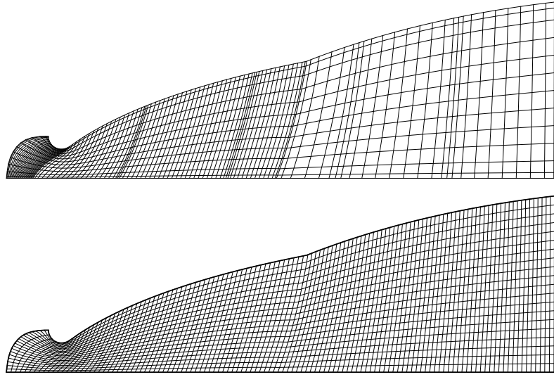
Fig. 12 Control points and harmonic mesh for the dual bell.
