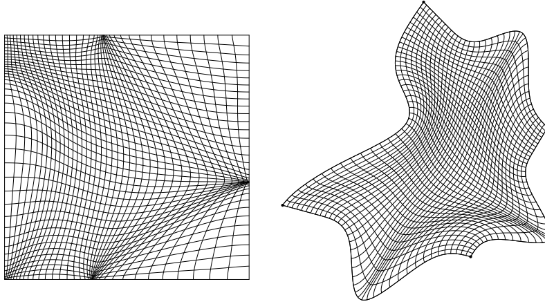
Fig. 15 Final grid with complete boundary control.
