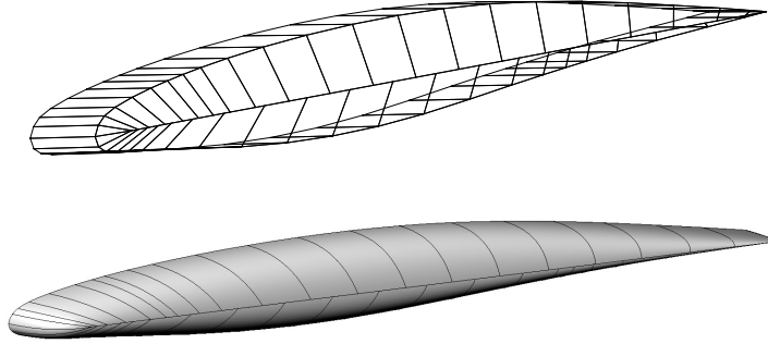
Fig. 8 Wing tip – Control points (top), knot-isolines (bottom).
