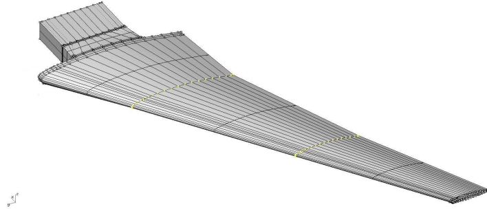
Fig. 2 View of the complete model with mounting unit.
