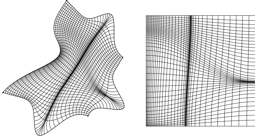
Fig. 14 Grid, orthogonal near the boundaries, and its control mapping
