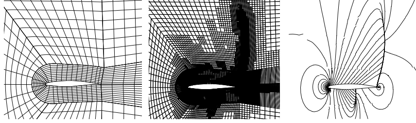
Fig. 1 Initial coarse grid, final adapted grid and pressure distribution for flow around BAC 3-11 profile, Mach 0.85.
