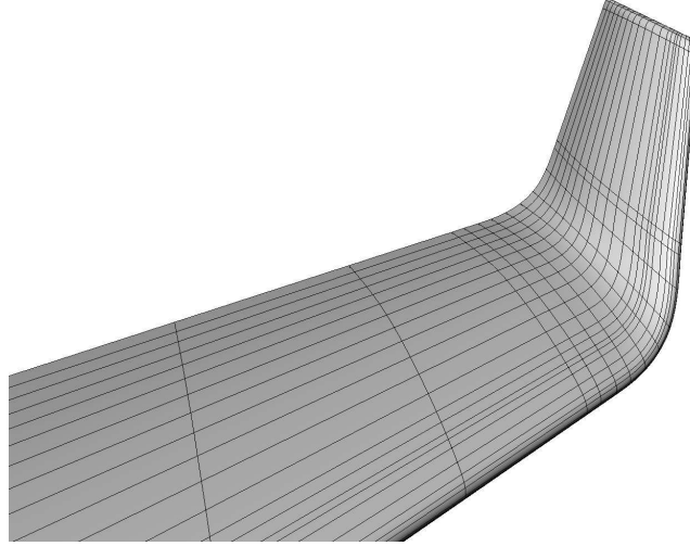
Fig. 11 Winglet with dihedral angle a = 10^\circ and bending angle w = 60^\circ .
