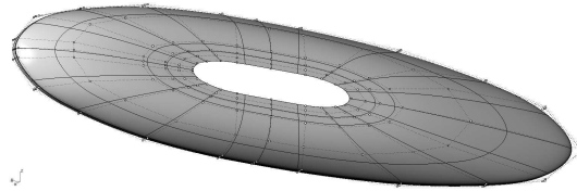
Fig. 3 Simplified fuselage – control points and knot-isolines
