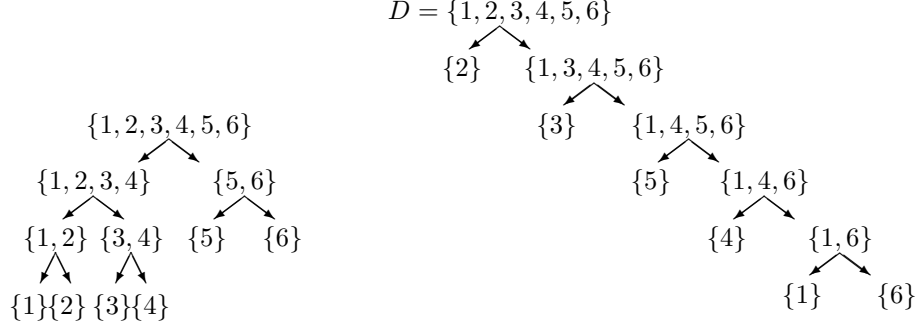
Figure 4: The example dimension tree for the hierarchical Tucker format (left) and one of the TT-trees where the node t = \{1, 4, 6\} and the corresponding rank appears (right).
