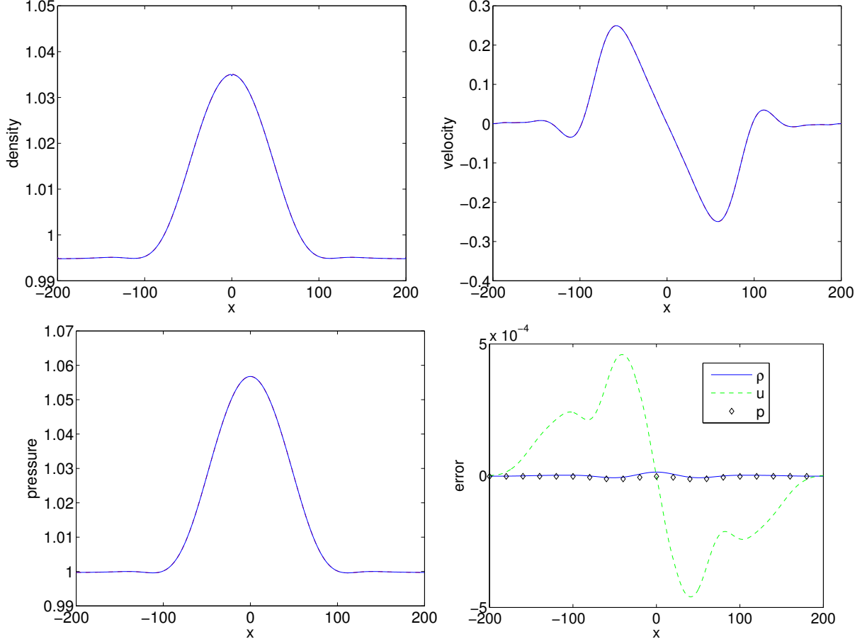
FIGURE 1. Two colliding acoustic pulses problem. Numerical solution for \varepsilon = 0.01 obtained by the second order scheme without any limiters, \hat{\nu} = 0.9 , \nu = 90 . The dashed lines represent the solution with 20 iterations and the straight lines show the solution without iterations. Top left: density. Top right: velocity. Bottom left: pressure. Bottom right: difference between density, velocity and pressure.
