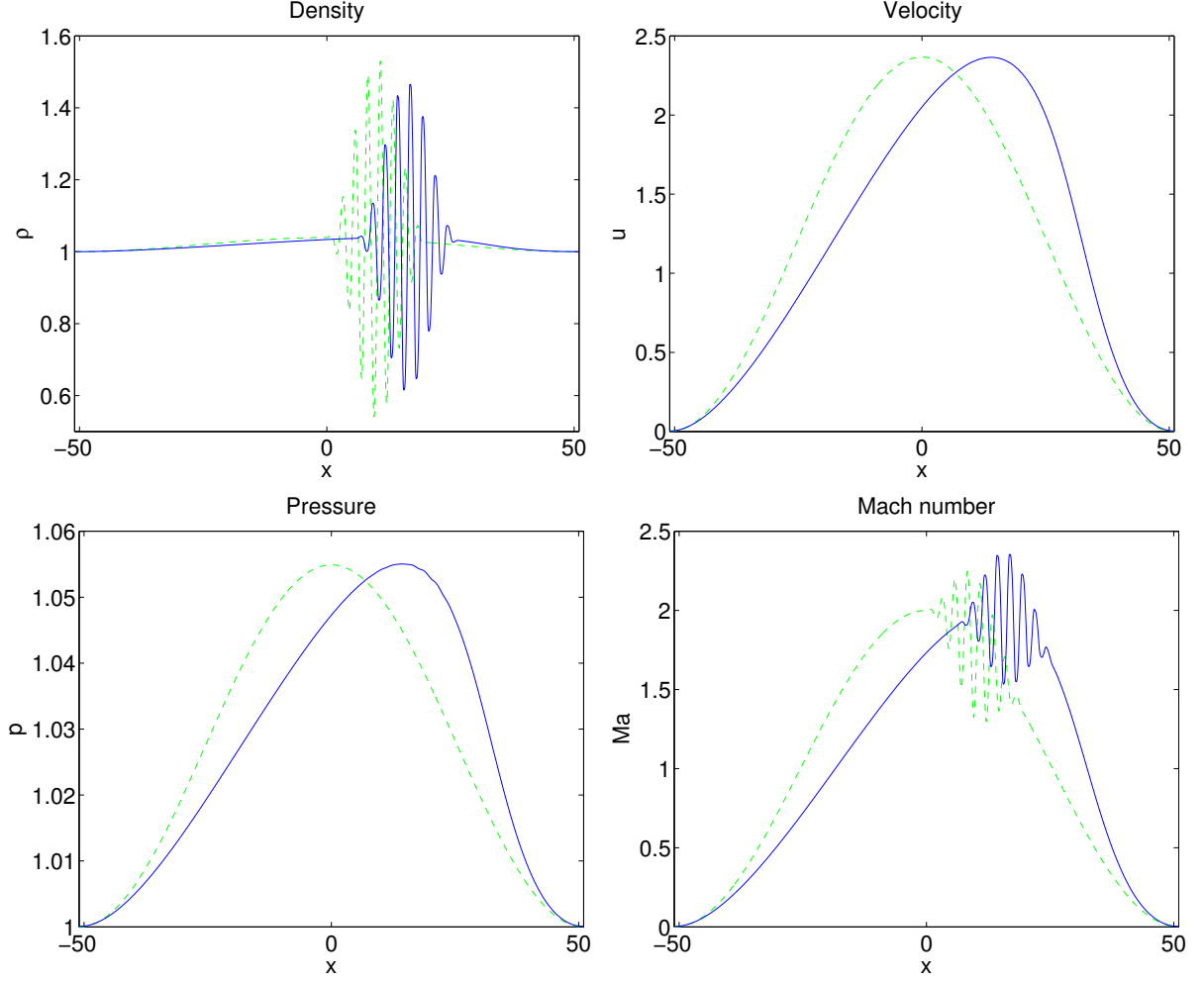
FIGURE 3. The results of density layering problem at t = 5.071 . Dotted lines: initial solution. Solid lines: solution obtained by the second order scheme. The CFL numbers are \hat{\nu} = 0.45 , \nu_{eff} = 22.95 and \varepsilon = 1/51 .
