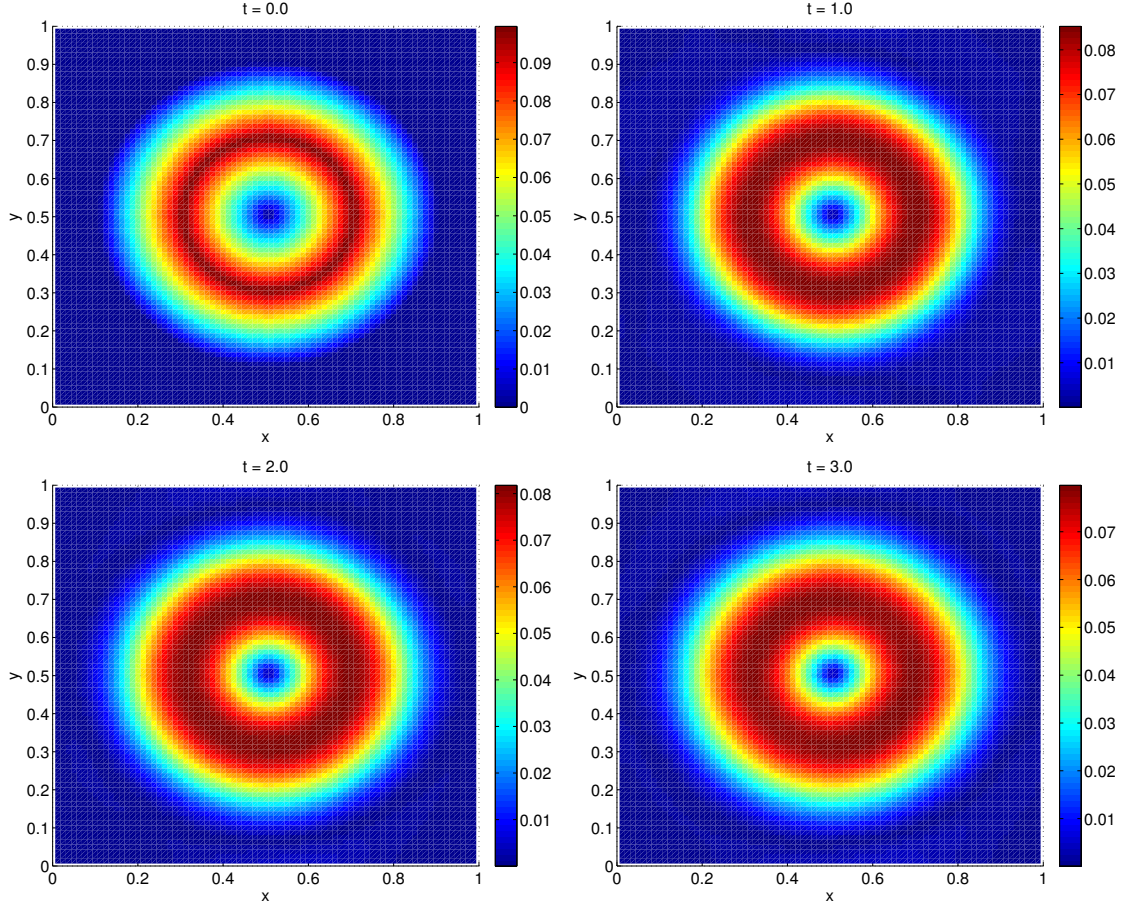
FIGURE 5. Gresho vortex problem: pseudo-colour plots of the Mach number at times t = 0, 1, 2, 3 . In this problem \varepsilon = 0.1 and the CFL numbers are \hat{\nu} = 0.45 and \nu_{eff} = 4.5 .
