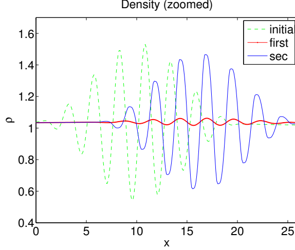
FIGURE 4. Density layering problem. Comparison of first and second order methods at t = 5.071 . \varepsilon = 1/51 , \hat{\nu} = 0.45 , \nu_{eff} = 22.95 .
