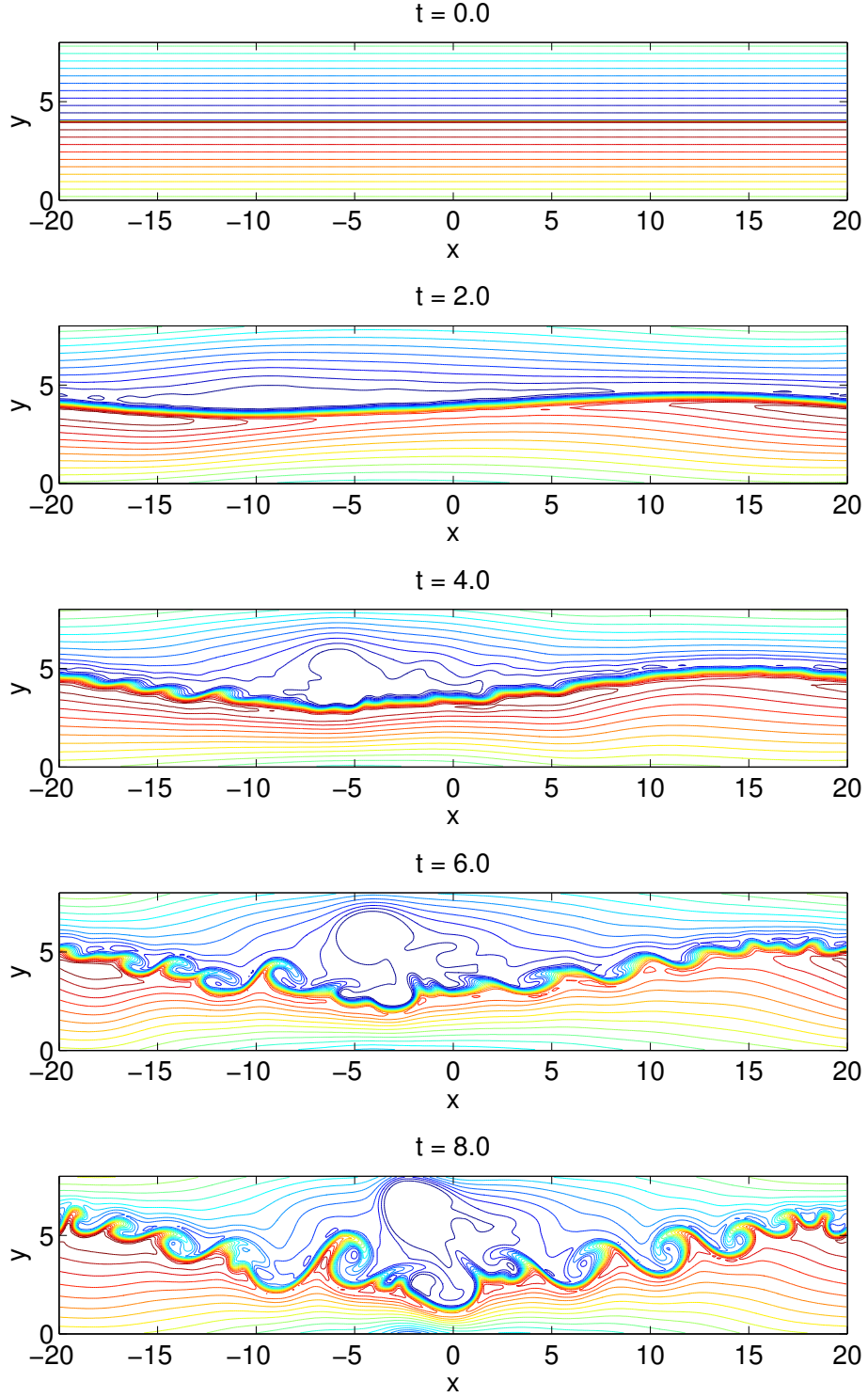
FIGURE 6. Baroclinic vorticity generation in weakly compressible flows. The isolines of the density at times t = 0, 2, 4, 6 . The CFL numbers are \hat{\nu} = 0.45 , \nu_{eff} = 9 and \varepsilon = 0.05 .
