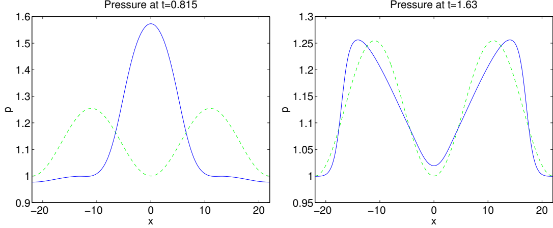
FIGURE 2. Two colliding acoustic pulses problem computed with the second order method. On the left: pressure distribution at t = 0.815 . On the right: pressure at t = 1.63 . Dotted line is the initial pressure distribution. Here, \varepsilon = 1/11 and \hat{\nu} = 0.9, \nu_{eff} = 9.9 .
