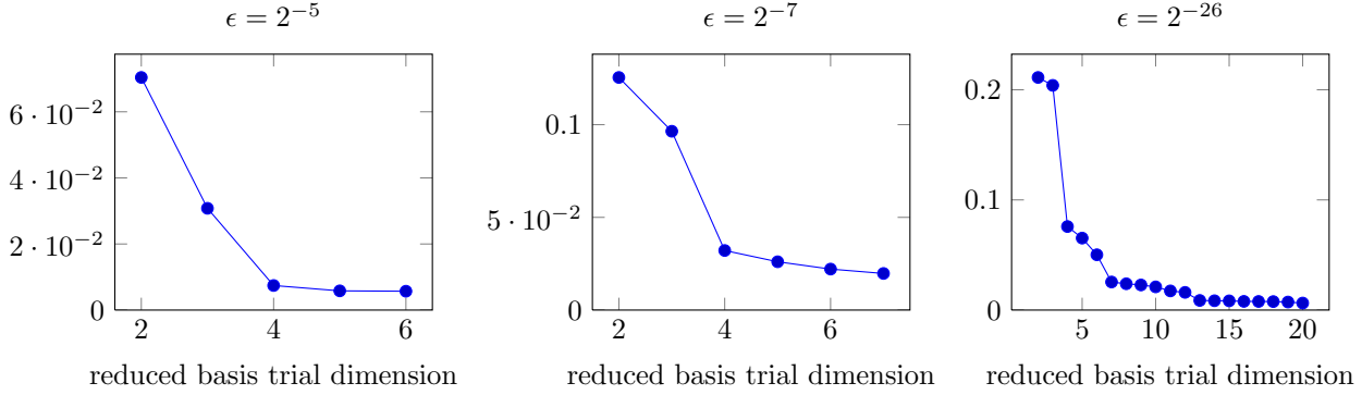
FIGURE 2. Surrogates of the reduced basis approximation for the convection-diffusion problem (6.7).
