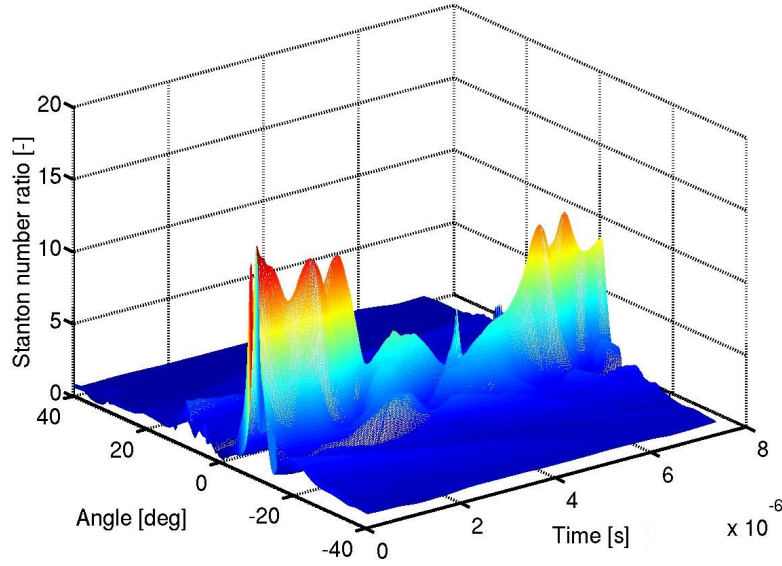
FIGURE 7. Stanton number distribution over time for the flow field illustrated in figure 3.
