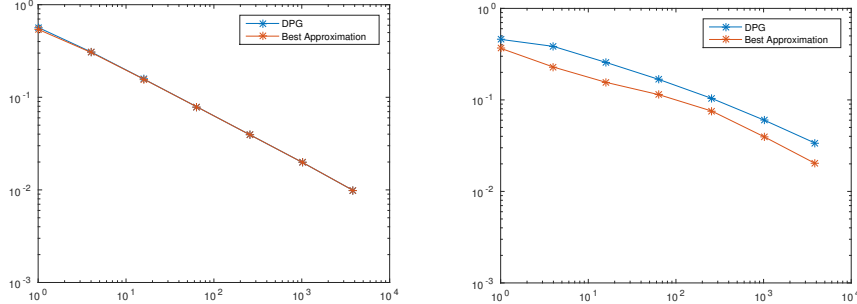
FIGURE 2. L_2(\Omega) -error in u_H and that in the best approximation versus 1/h^2 , for f(\mathbf{x}) = 1 - x_1 , \mathbf{b} = (1, 1)^\top (left) and \mathbf{b} = (1, \frac{1}{16})^\top (right).
