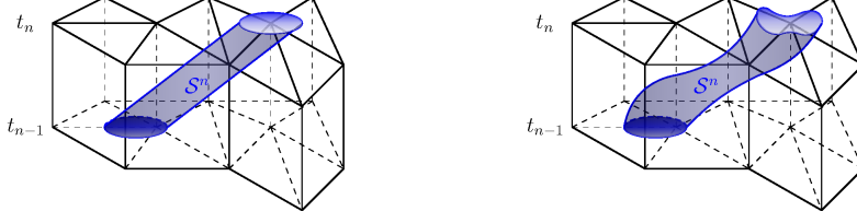
FIG. 3.1. Illustration of the local space-time triangulation \mathcal{Q}_n^S in one time slab. In the left picture we have a constant \mathbf{w} , hence (2.13) is satisfied.
