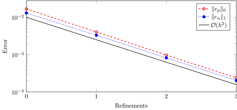
FIG. 7.1. Discretization errors for simultaneous temporal and spatial refinement.
